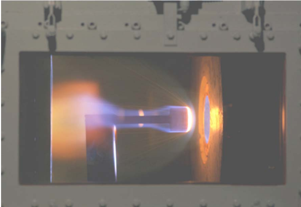
Figure 17O-2 Testing Thermal Insulation in a Wind Tunnel
