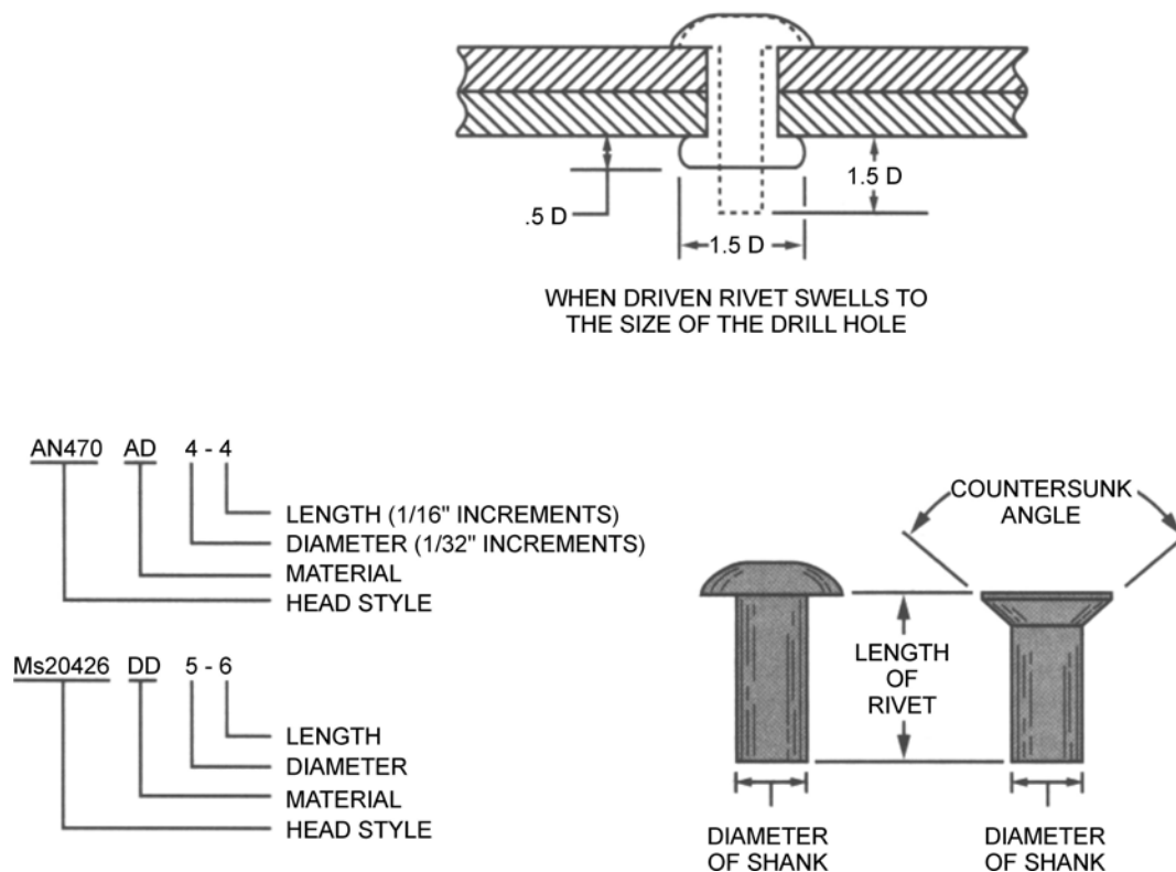
Figure 17S-6 Rivet Applications, Dimensions and Designations
