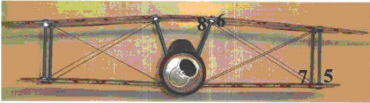
Figure 17AG-5 Flying Wires
